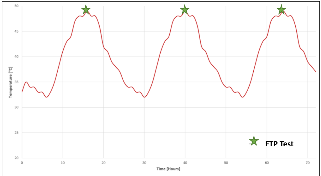
Operation High Temperature Test Profile
