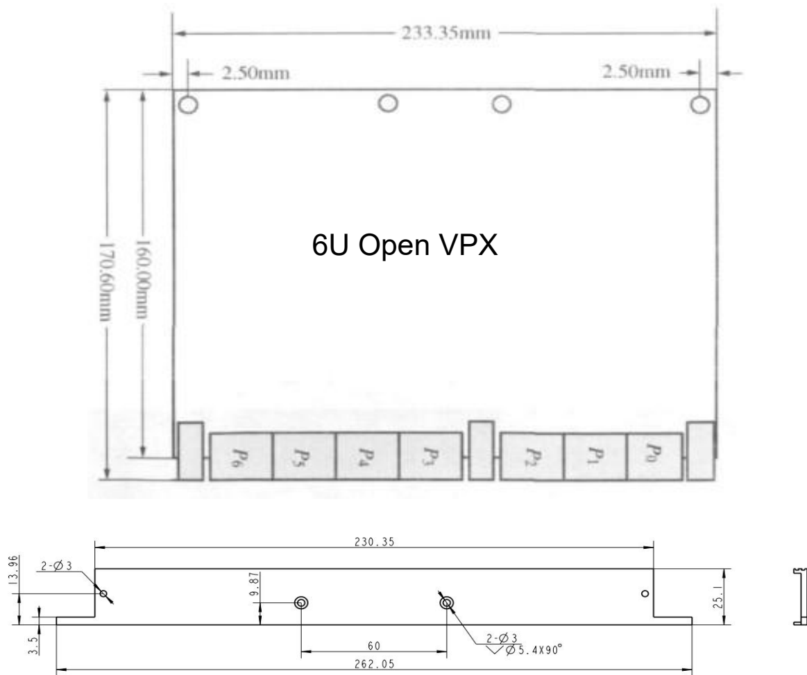
Figure 2: 6U VPX mechanical dimension
