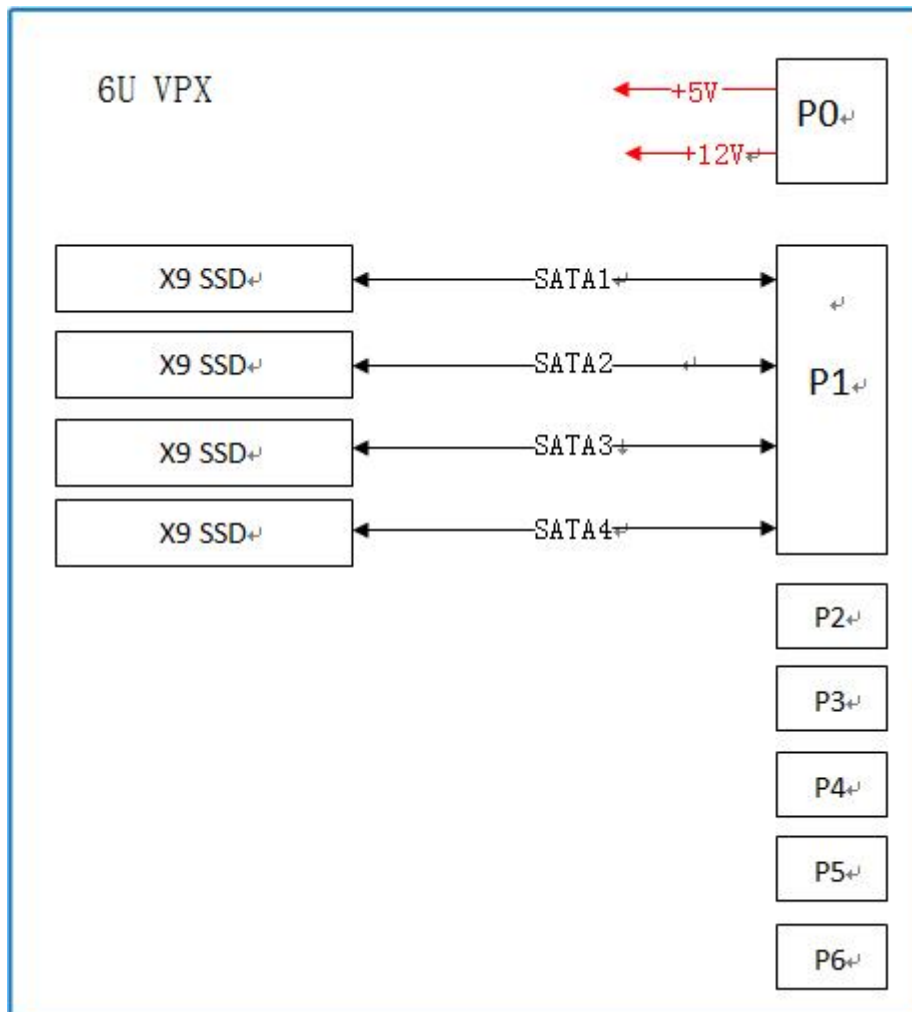
Figure 1: Renice VPX (4 channels X9 SSD ) Block Diagram
